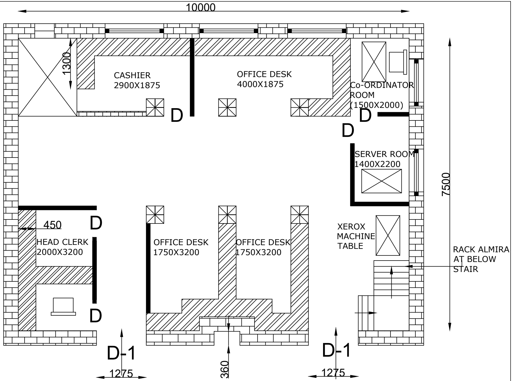
PROPOSED OFFICE INTERIOR PLAN FOR OFFICE AT MAHARAJA MANINDRA CHANDRA COLLEGE
